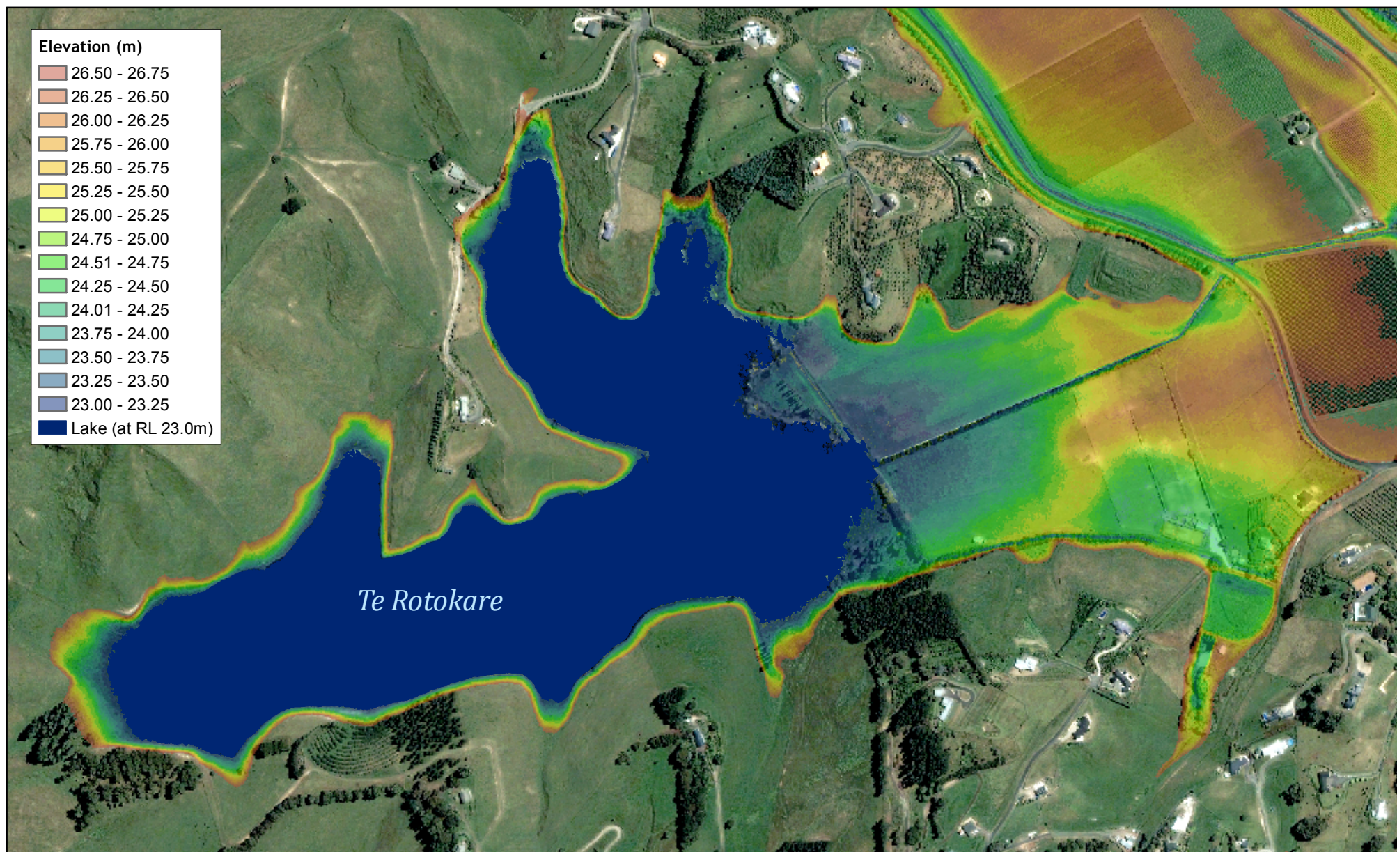
Figure 4. Topography of floor of Te Rotokare basin and margins of lake
