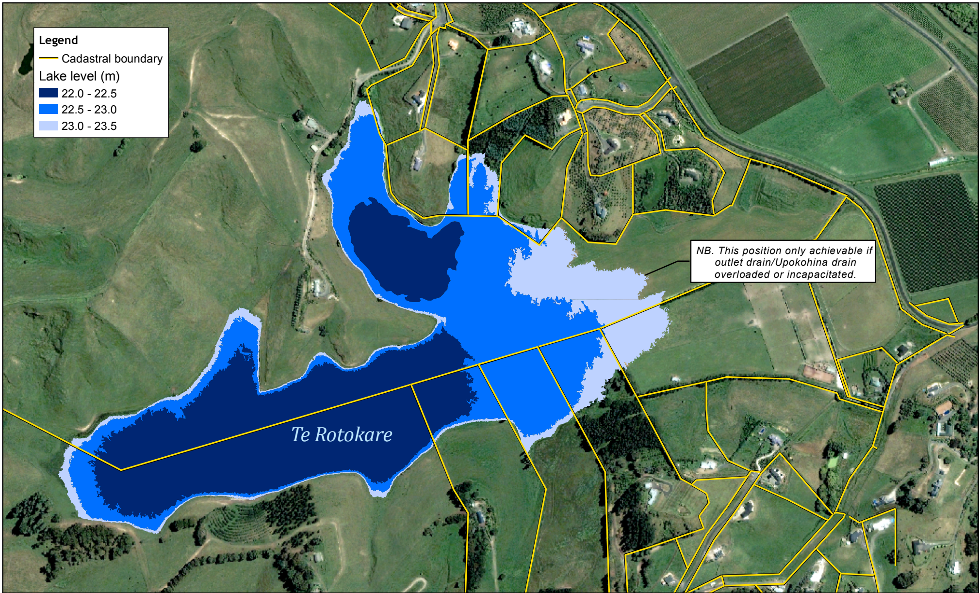
Figure 7. Footprint of Te Rotokare at three nominal lake levels
