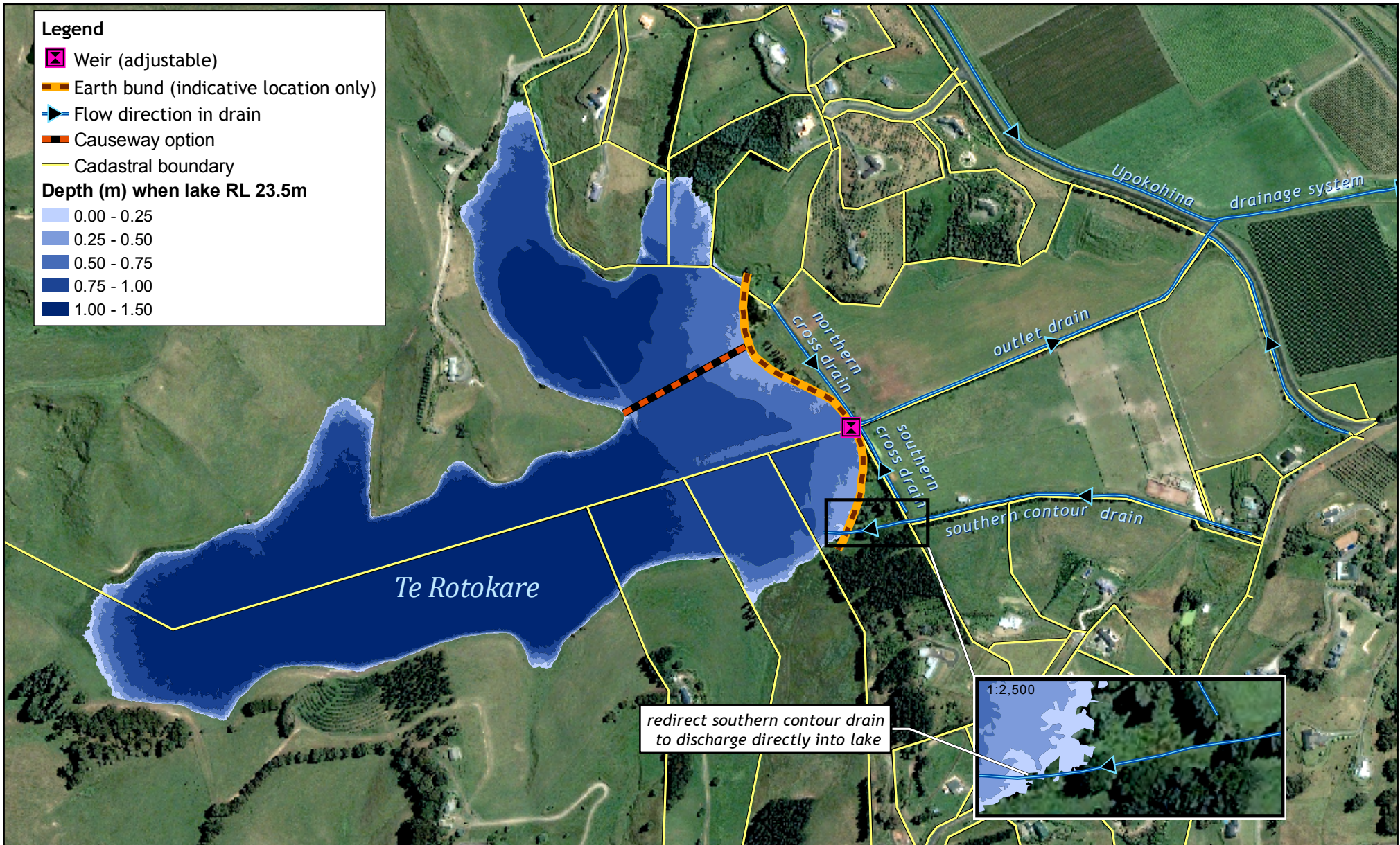
Figure 9. Recommended hydrological enhancement option for Te Rotokare and resulting bathymetry
