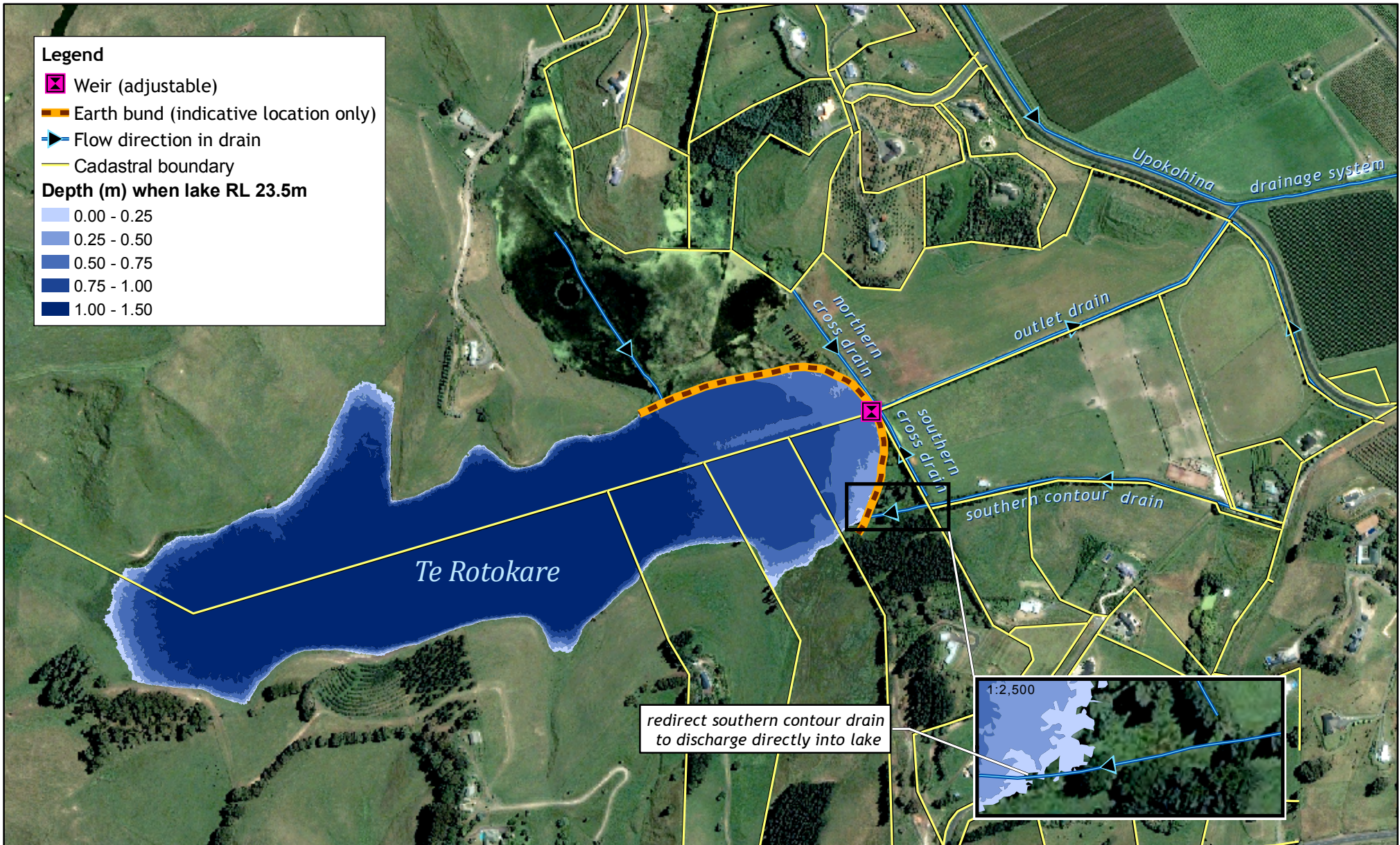
Figure 8. Hydrological enhancement option for main body of Te Rotokare only, and resulting bathymetry
